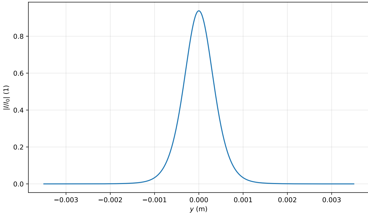
Intensity profile I(x=0, y, z=2.627)/I_0 , P_{in}=0.7P_{cr} , artificial time
